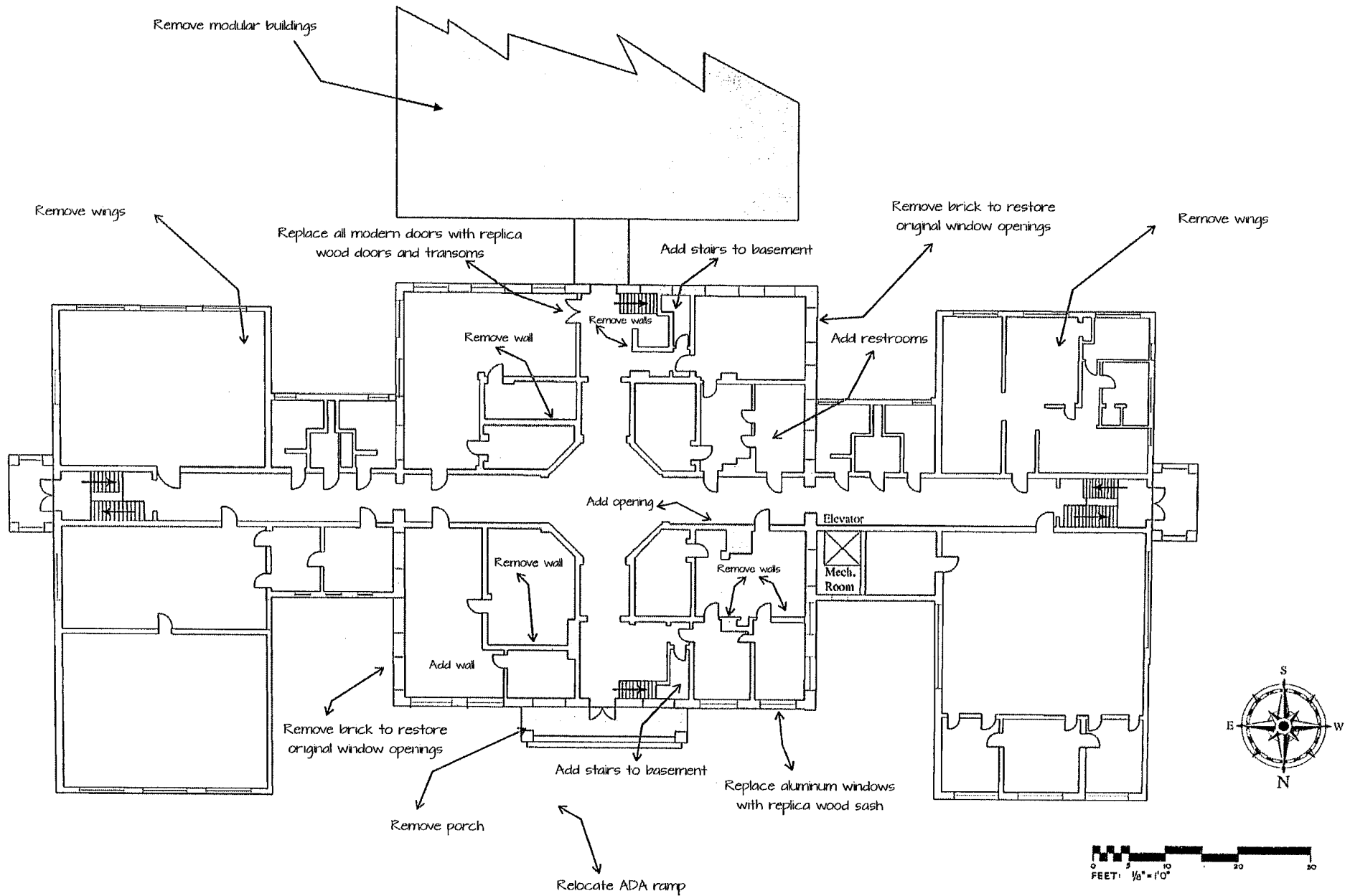
SANTA ROSA COUNTY COURTHOUSE EXISTING FIRST FLOOR PLAN
