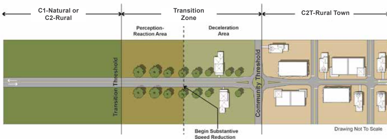
FIGURE 4-8 TRANSITION ZONE FROM C1-NATURAL/C2-RURAL TO C2T-RURAL TOWN CONTEXT CLASSIFICATION
